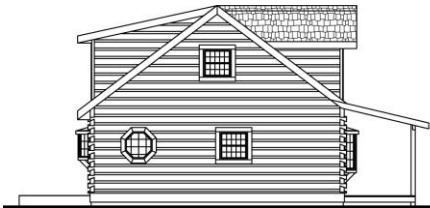
LEFT ELEVATION 40'-0"
